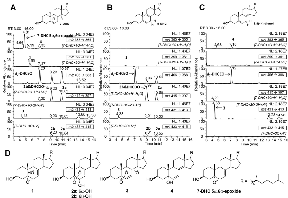
Figure 1. Normal phase HPLC-APCI-MS-MS analysis of oxysterols formed from free radical oxidation of 7-DHC (A), 8-DHC (B), and cholesta-5,8(14)-dienol (C). (D) Major oxysterols identified. D -3,5-dihydroxycholest-7-en-6-one (DHCEO) was added to each sample as a standard for proper comparison of the retention times between different chromatograms. The parent ion of each chromatogram and the MS/MS transition were marked in the corresponding MS panel.
